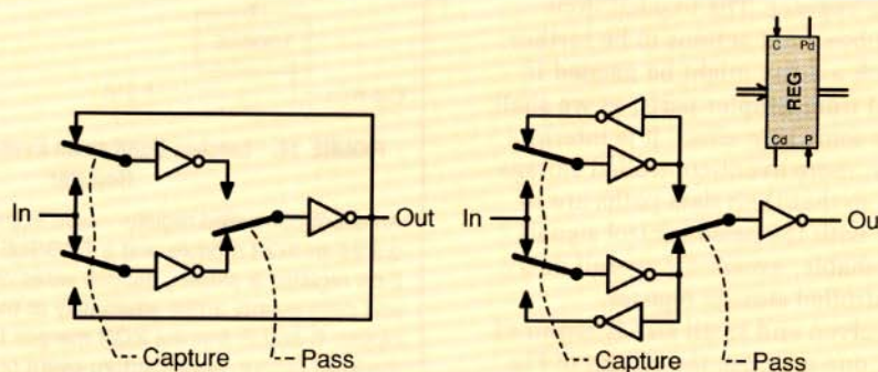
FIGURE 12. Event-Controlled Storage Elements
